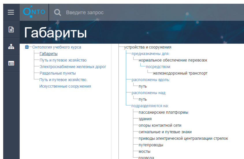
Fig. 1. A piece of Clearance Limits ontology in CRuL
